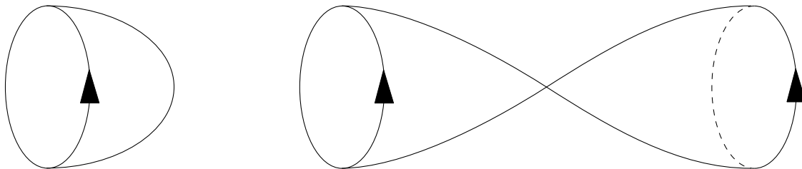
Figure 3. These graphs are the would-be leading contributions of respectively \langle \text{tr } \Omega \rangle_{\text{YM}} and \langle (\text{tr } \Omega)^2 \rangle_{c,\text{YM}} . They are forbidden by the topology of the thermal dimension.
