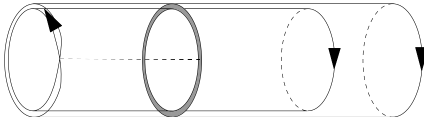
Figure 7. The connected expectation value \langle \text{tr } U(\omega_1) \text{tr } U(\omega_2) \text{tr } U(\omega_3) \rangle_{YM,c} with w_1 = w_2 = 1 , w_3 = -2 . The four-link integration in the gray area makes vanish this contribution, as explained in eq. (A.8).
