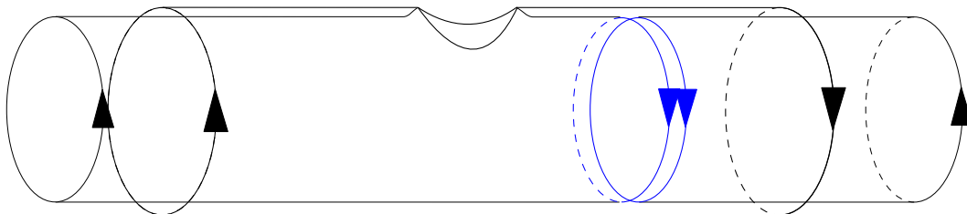
Figure 5. This graph is a leading contribution of \langle (\text{tr } \Omega)^3 \text{tr } \Omega^\dagger \rangle_{c,S/AS} . The pair of blue loops represent the insertion of a vertex \text{tr } R[U(\omega)] , due to the derivative with respect to c(\omega) .
